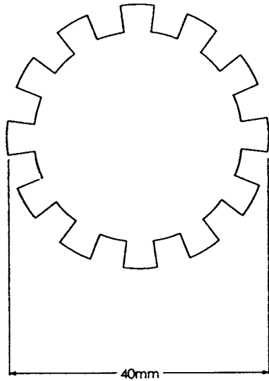
NOTE—Dimensions are given in millimetres. FIG. 2 Distributor Plate
